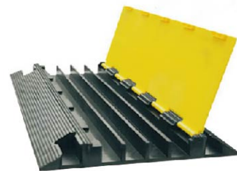
Four Channel Model:CP-04 Size:900X500X60mm Channel Size:40X45mm Weight:14KG
