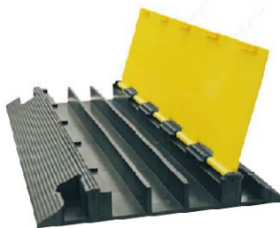
Three Channel Model:CP-03 Size:900X500X70mm Channel Size:55X65mm Weight:14.5KG
