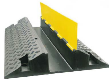
Large-One Channel Model:CP-01L Size:1000X580X125mm Channel Size:110X125mm Weight:22KG
