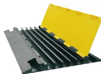
Five Channel Model:CP-05 Size:900X500X50mm Channel Size:30X40mm Weight:13KG
